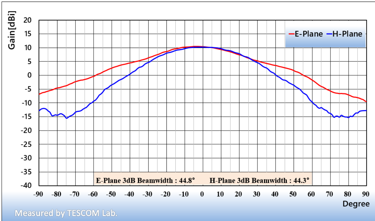
<TC-93474A Port 1 @ 24 GHz>
