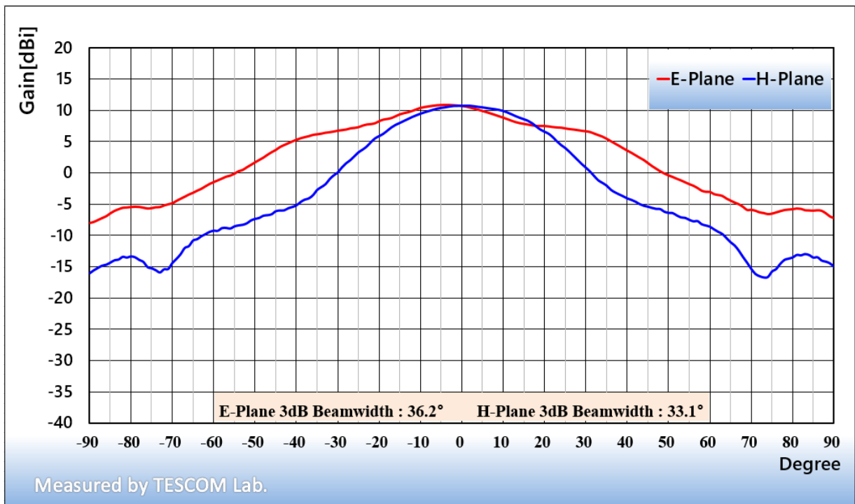
<TC-93474A Port 1 @ 28 GHz>
